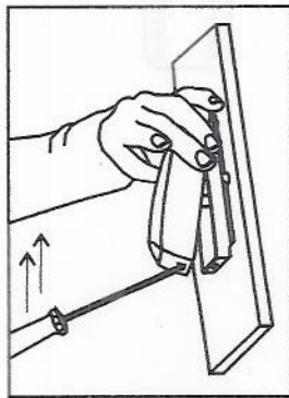
Insert a small 1-1.5mm flat screw driver into the slot at the back of the housing and lever the lid open.
